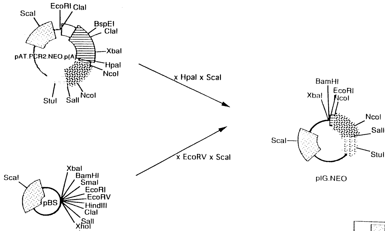
Fig. 5 Construction of pIG.NEO
